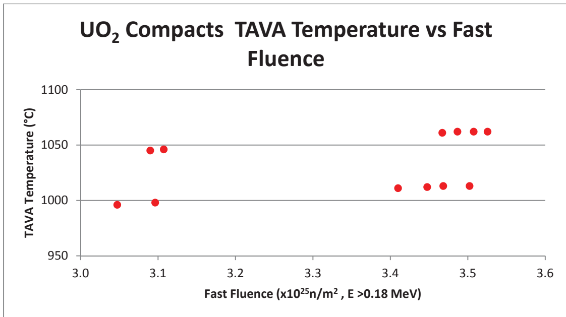
Figure 24. Time-average volume-average temperature ( ^{\circ}\text{C} ) vs. Fast neutron fluence ( E > 0.18 \text{ MeV} ) for AGR-2 compacts.
