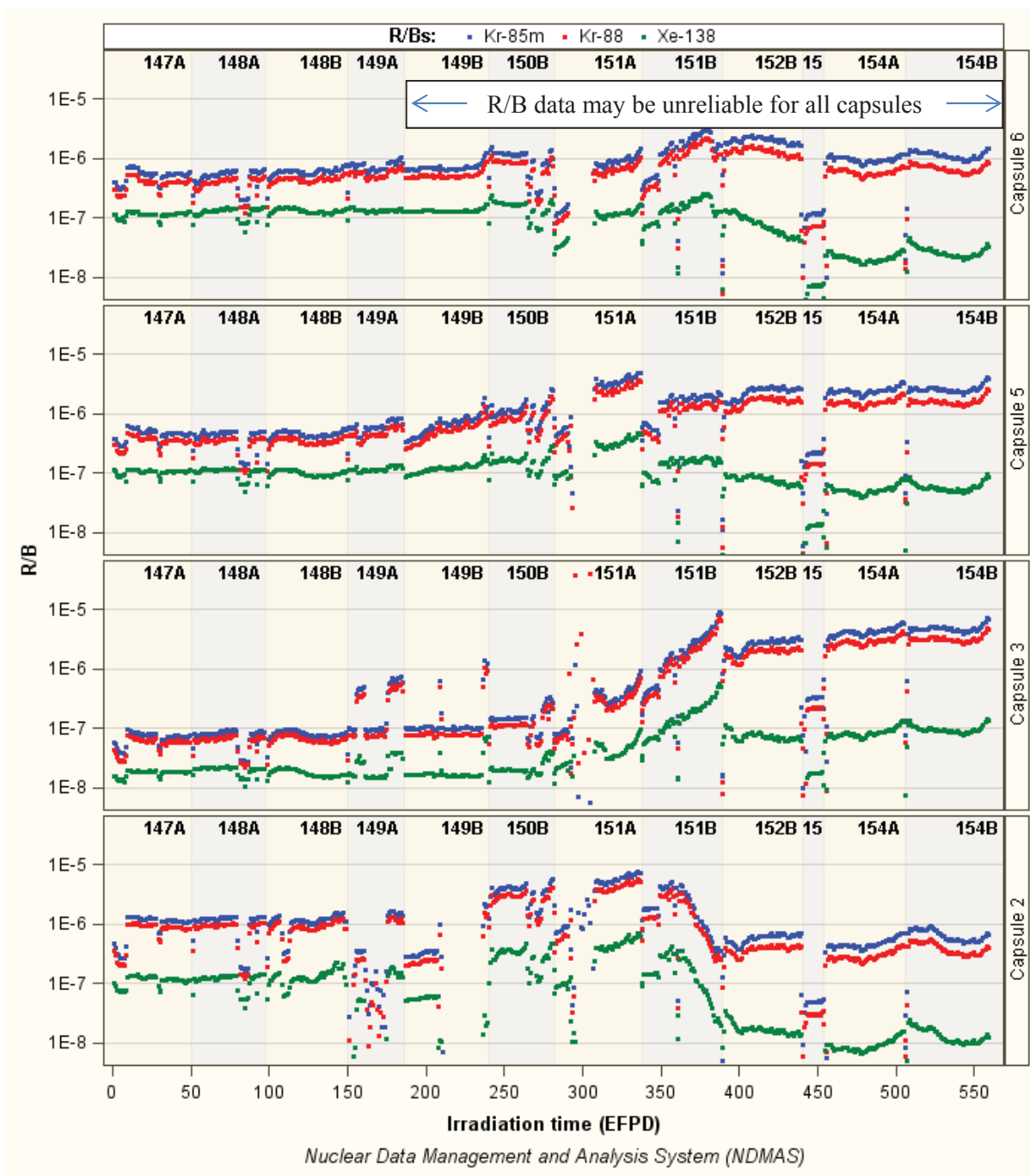
Figure C-1. Unfiltered R/B ratios from daily birthrates for Kr-85m, Kr-88, and Xe-138 versus time in EFPD. Data from Cycle 149A and following cycles are not deemed reliable because of gas flow and cross-talk issues.
