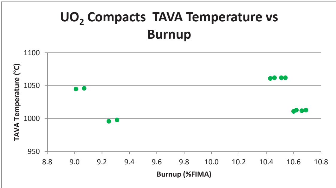
Figure 23. Time-average volume-average temperature (°C) vs. Burnup (%FIMA) for AGR-2 compacts.
