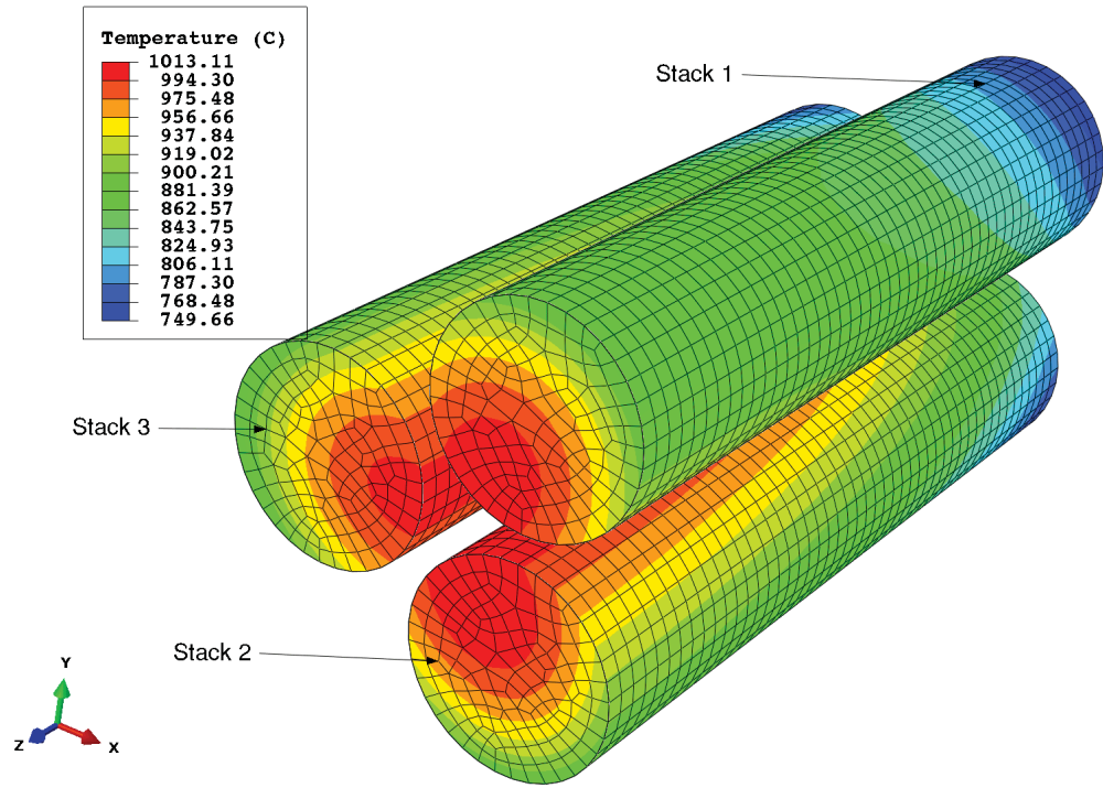
Figure 14. Temperature (°C) contour plot cutaway view of the three fuel stacks.
