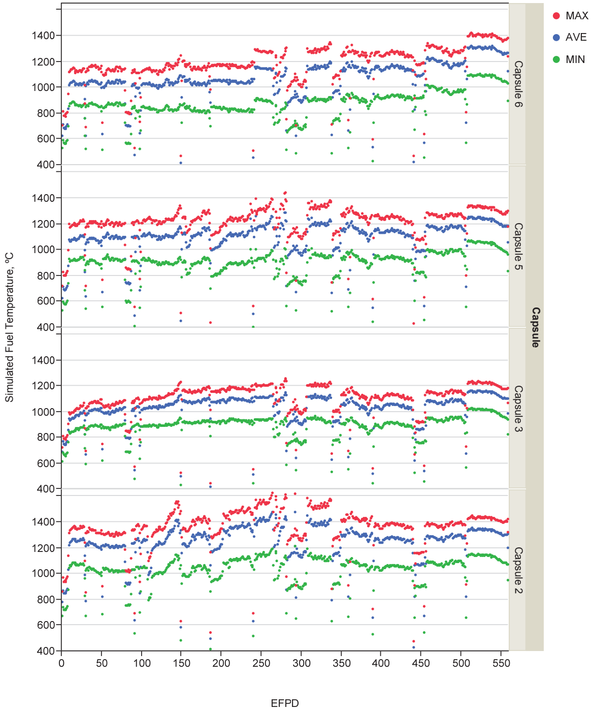
Figure 15. Calculated daily minimum, maximum, and volume-average temperatures.
