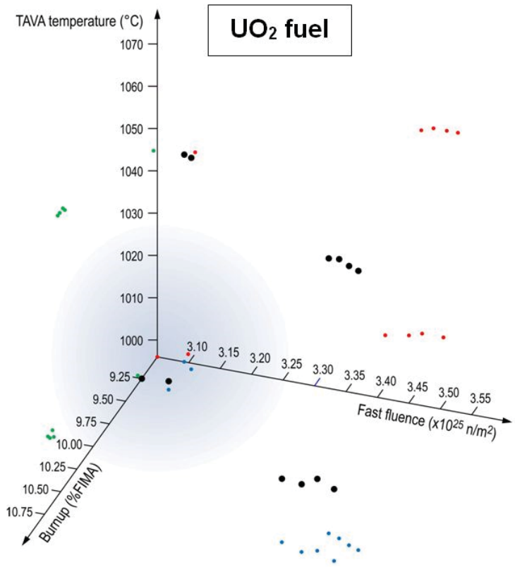
Figure 22. 3-D scatter plots of the irradiation characteristics of the AGR-2 compacts.
