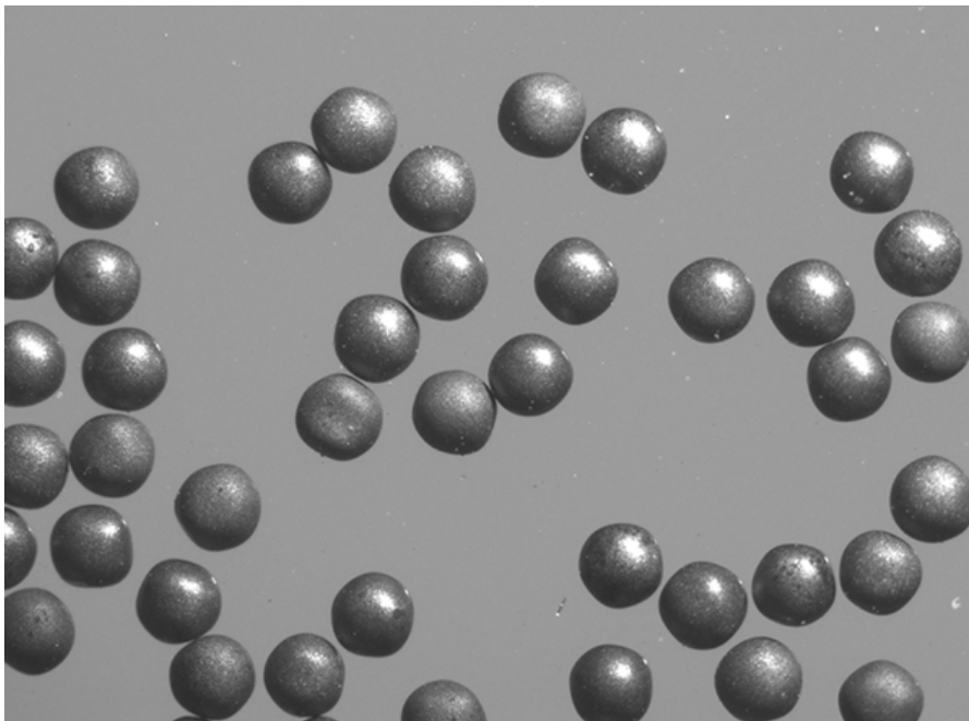
TRISO particles
