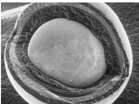
TRISO particles
