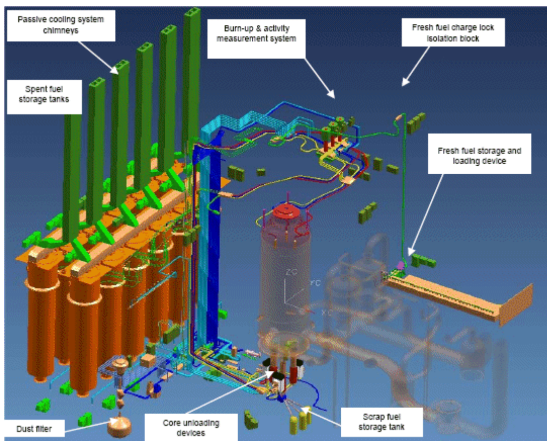
Figure 6-2. PBMR-400 fuel handling and storage system [Ref. 34]
