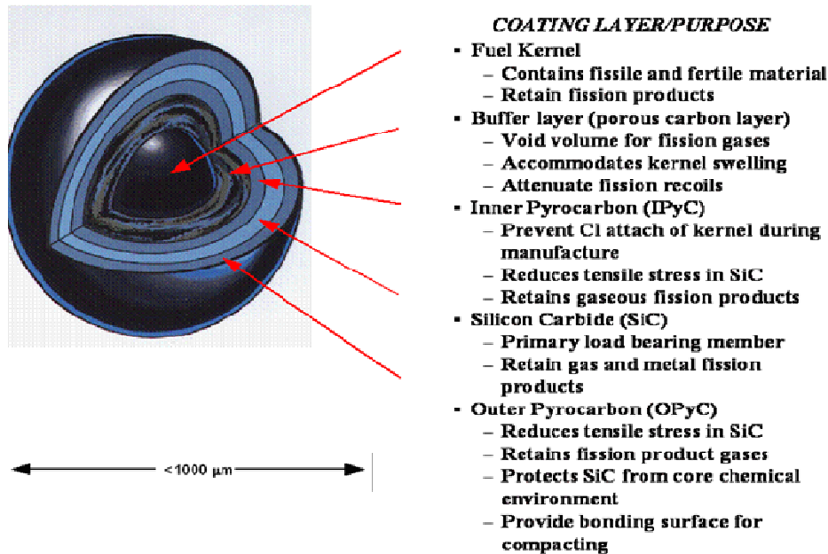
Figure 11. TRISO fuel particle configuration and coating purposes.
