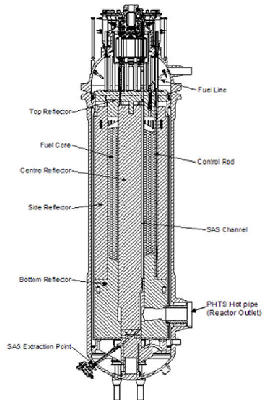
Annular Pebble Bed Reactor
