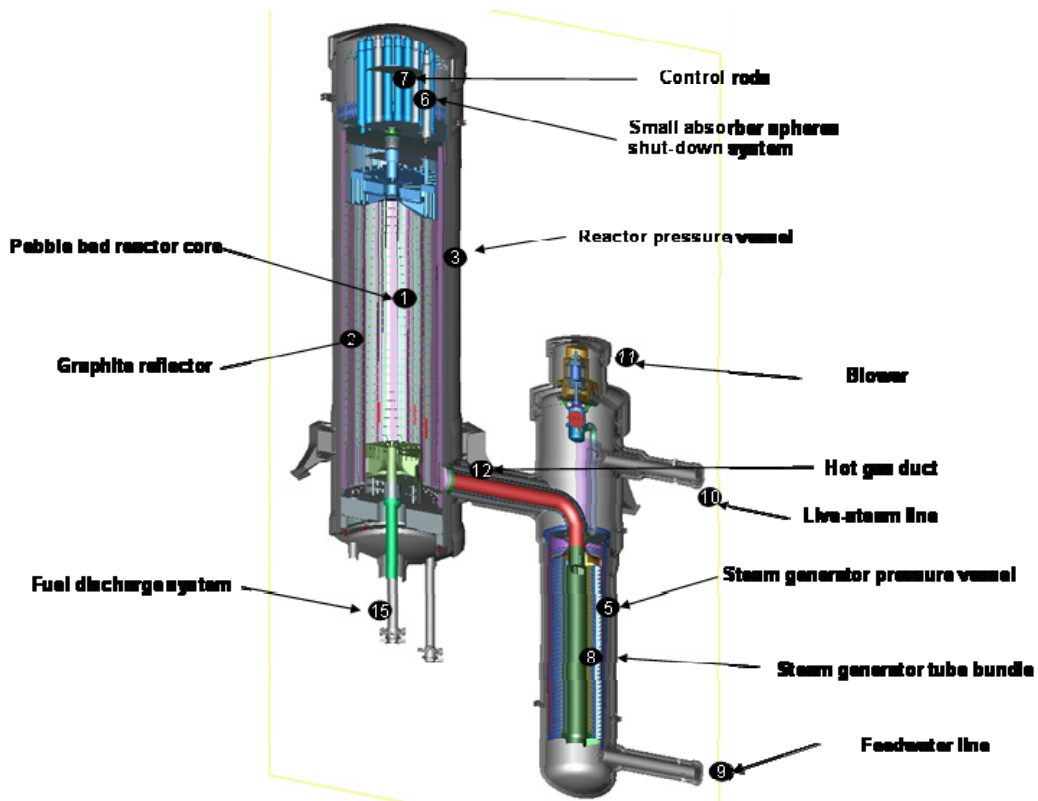
Figure 7. WEC/PBMR team commercial plant configuration.
