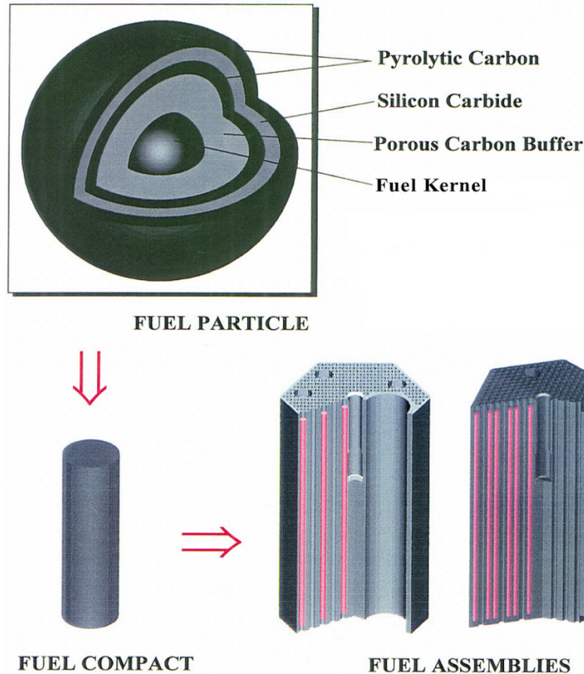
Figure 12. Prismatic reactor fuel particles, compacts and assemblies.
