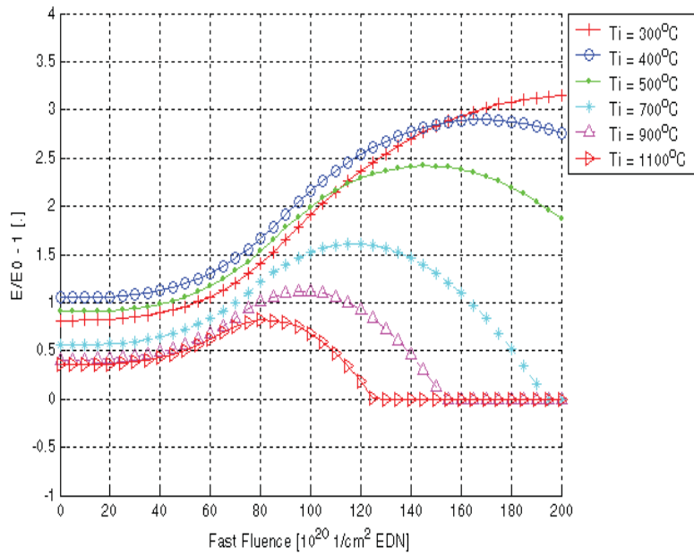
Figure B-8. Typical irradiation-induced modulus changes in reactor graphite.
