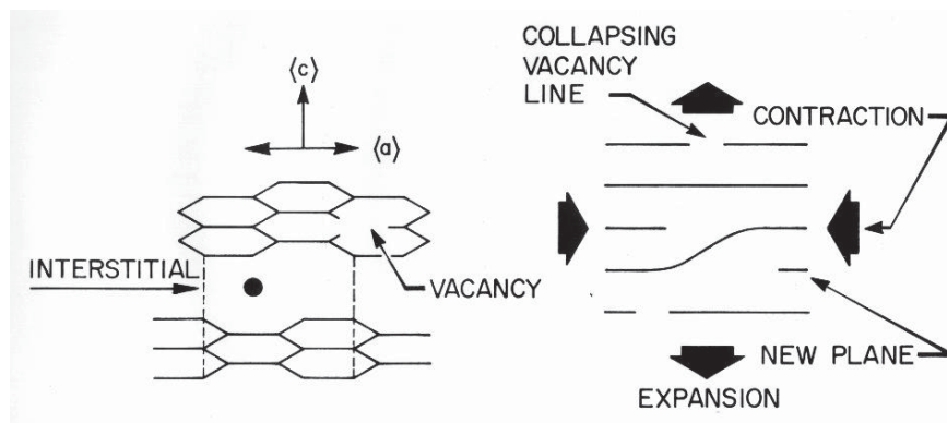
Figure B-2. Neutron irradiation damage mechanism illustrating induced crystal dimensional changes.
