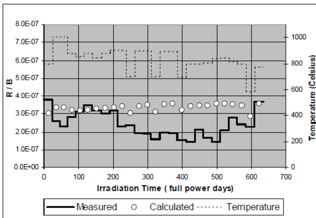
Figure 4-10. Measured and calculated ^{135\text{m}}\text{Xe} R/B comparison for test element C1K6.
