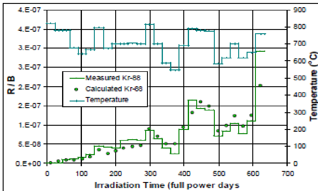
Figure 4-7. Measured and calculated ^{88}\text{Kr} R/B comparison for test element B1K6 (contamination release).
