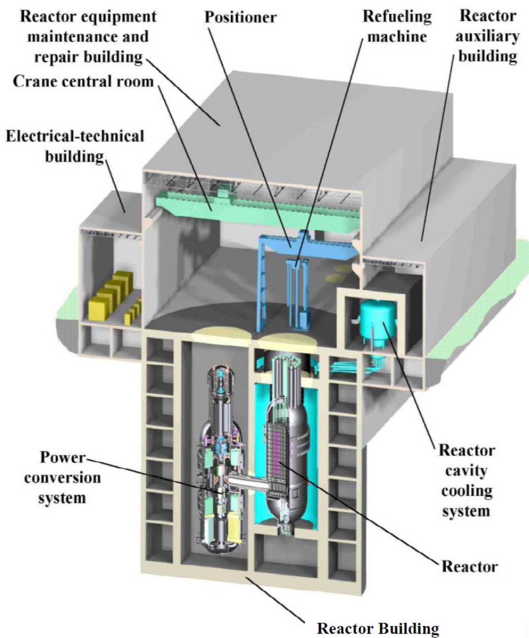
Figure B-4. Prismatic reactor building conceptual configuration.
