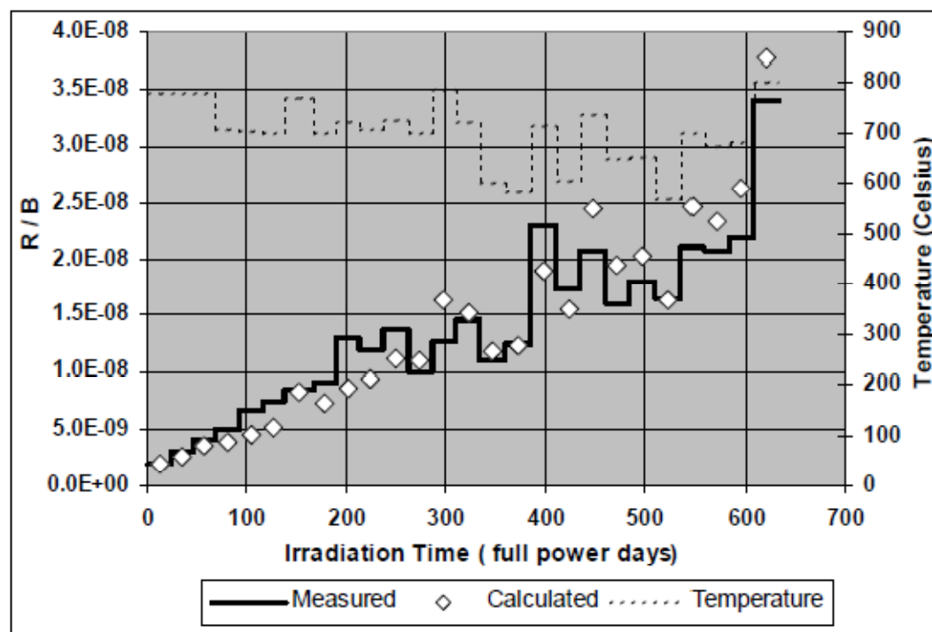
Figure 4-8. Measured and calculated ^{135\text{m}}\text{Xe} R/B comparison for element B1K6 (contamination release).
