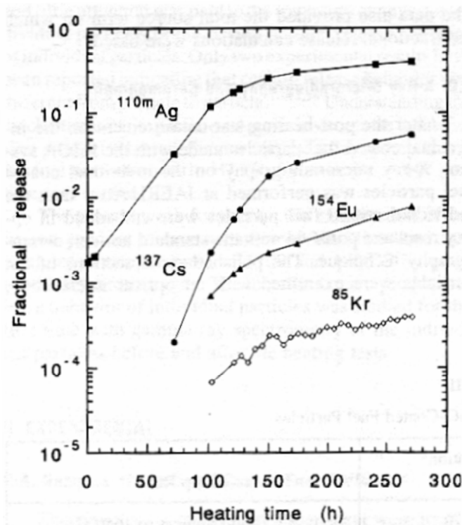
Figure C-3. Metal release during post-irradiation heating of HRB-22 particles at 1700°C.
