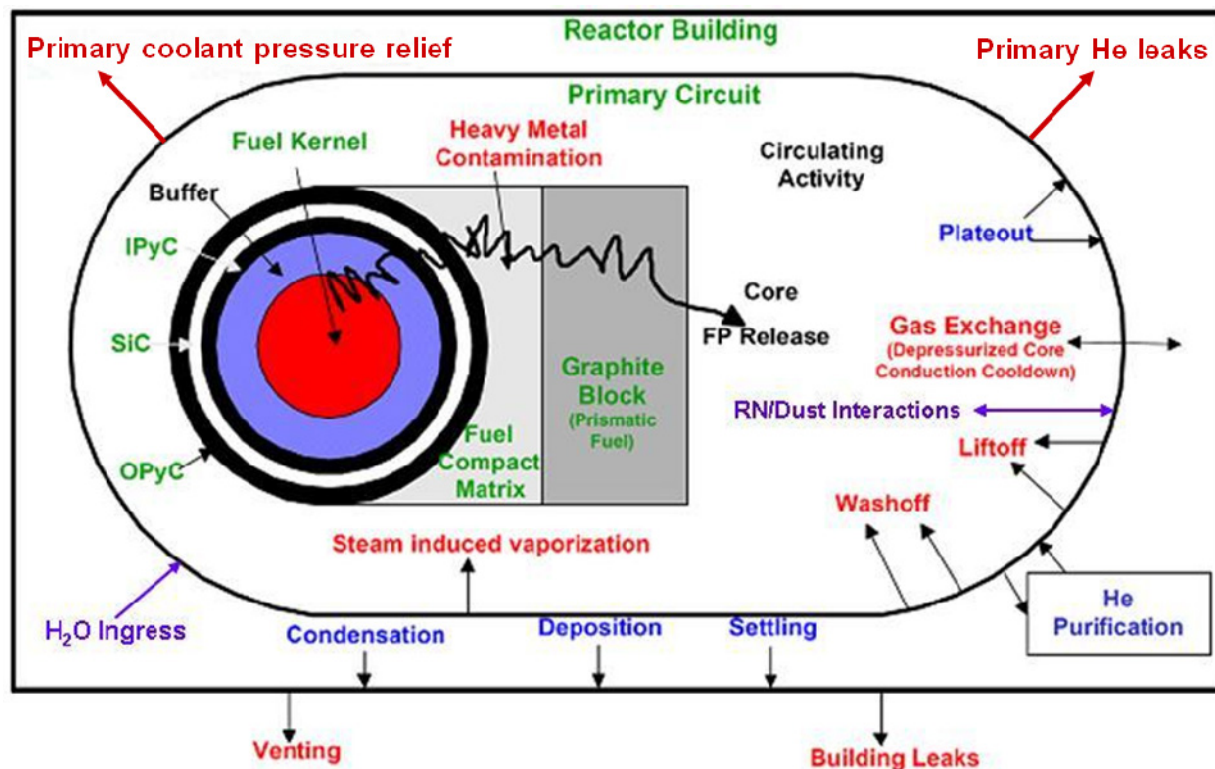
Figure C-1. HTGR radionuclide retention system.
