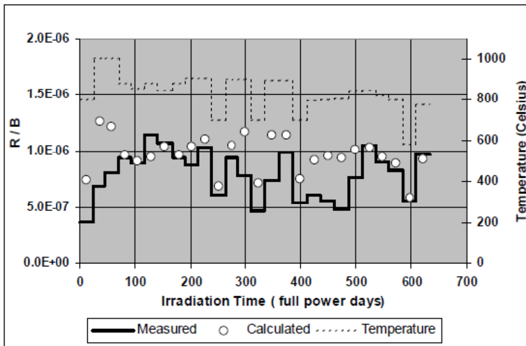
Figure 4-9. Measured and calculated ^{88}\text{Kr} R/B comparison for test element C1K6.
